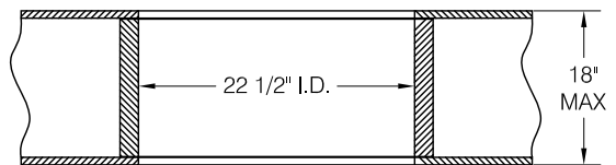
CAD: 24RUFN-SIDE-X.DWG
